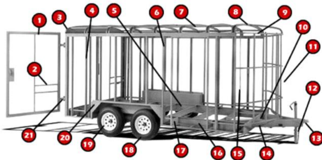
Fig. I.2: 1. Frame of rear door, 2. interior frame of door, 3. corner post, 4. vertical post, 5. cross-wise I beam, 6. wall studs, 7. roof runner, 8. roof bow, 9. front frame, 10. front and rear end rails, 11. nose frame or bulkhead, 12. approved safety chains, 13. lock ball coupler hitch, 14. trailer draw bars, 15. internal wiring, 16. length wise I beam, 17. cross-wise I beam, 18. tire, 19. wheel, 20. protective tire fender, 21. hinge for rear door.
