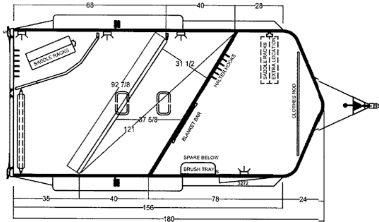
Fig. I.17: An example of a simple slant-load, two-horse, tag-along type trailer with a small tack and dressing room in front. Various designs can induce a variety of challenges under overturn or wreck conditions, and maximum access and egress methods to the horses is preferred.
