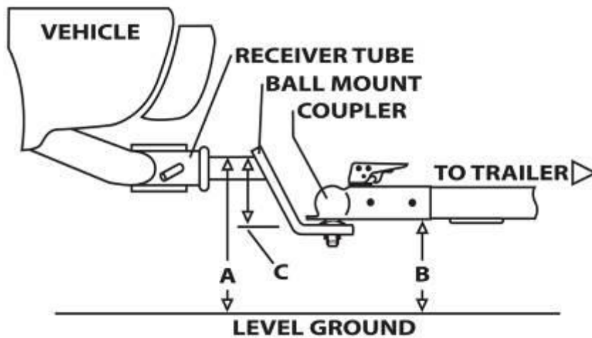
Fig. I.11: A leveler “bumper pull” or “tag along” hitch showing the coupler latch, but no receiver pin or chain connections are indicated. curtmfg.com
