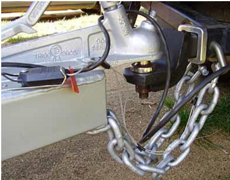
Fig. 32.1: Heavy chains help guard against complete separation of the trailer from the tow vehicle but do not offer directional control. Chains must be maintained, and should be correctly attached to both the tow vehicle and trailer. While it is illegal to improperly hitch a trailer, hitch parts are not standardized for non-commercial use. Components may be recommended by guess-and-by-gosh and “nobody ever complained” at a dealership. It is always worthwhile to consult a trusted, certified mechanic who takes a keen, searching interest in these things or a dedicated professional association.
