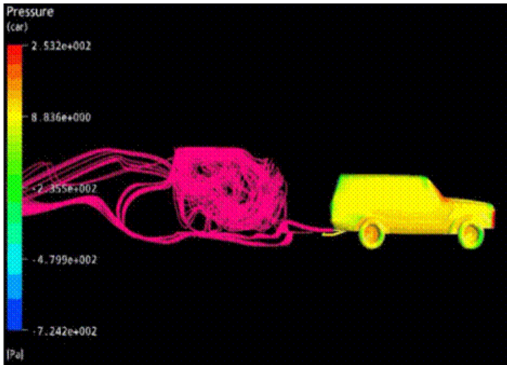
Fig. 12.1: At forty miles per hour with a light crosswind, exhaust (pink lines) fills the trailer. Exhaust patterns depend on tow vehicle shape as well as prevailing crosswinds. Exhaust seeps up through the floor, the front ventilation, and may be sucked into the open back.
